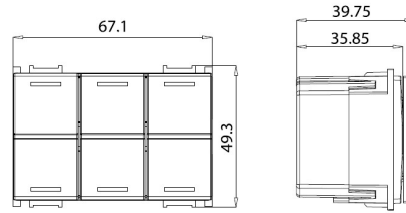
3 Gang 3M Mechanism Dimension:
