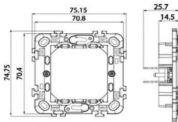
2M Mounting Frame Dimension:
