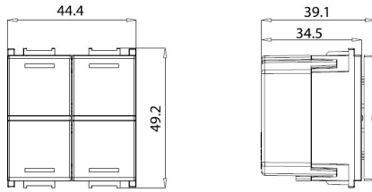
4 Gang 2M Mechanism Dimension:
