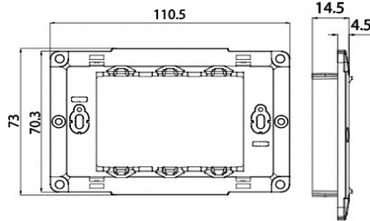
3M Mounting Frame Dimension:
