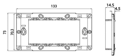
4M Mounting Frame Dimension:
