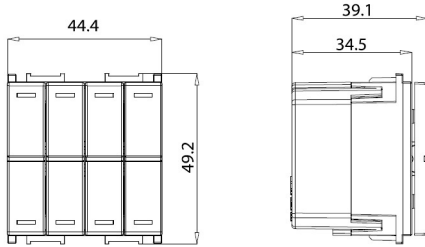
2M Mounting Frame Dimension:
