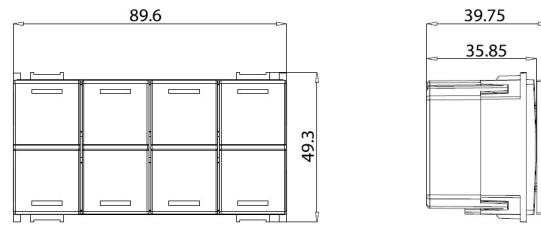
4 Gang 4M Mechanism Dimension:
