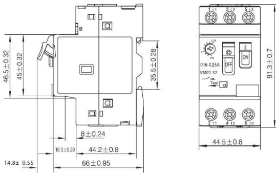
VMP2-32 (0.16-32A)
