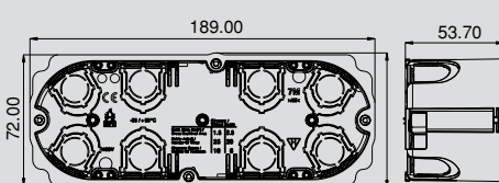
Hollow Wall Box 7M
