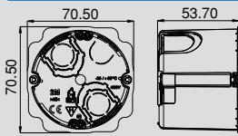
Hollow Wall Box 2M
