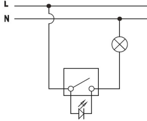
Circuit Diagram for Switch
