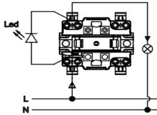
Circuit Diagram for Switch
