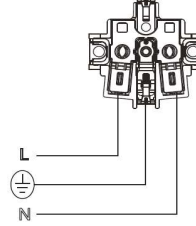
Circuit Diagram for Socket
