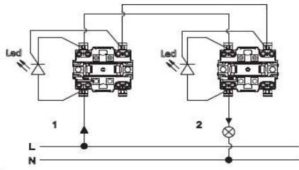
Circuit Diagram for Switch
