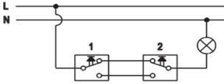
Circuit Diagram for Switch
