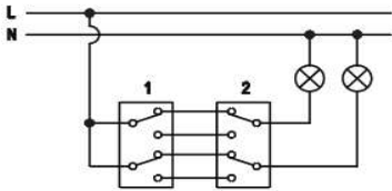
Circuit Diagram for Switch
