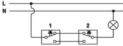
Circuit Diagram for Switch
