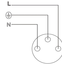
Circuit Diagram for Socket
