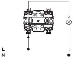
Circuit Diagram for Switch
