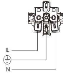
Connection Diagram for Socket
