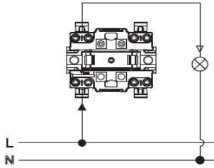
Connection Diagram For Switch
