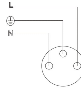
Circuit Diagram for Socket
